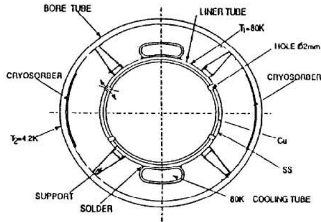
Figure 1. SSC Dipole Liner System.
