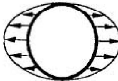
Figure 3. Eddy Current Pressure at Copper Liner.
