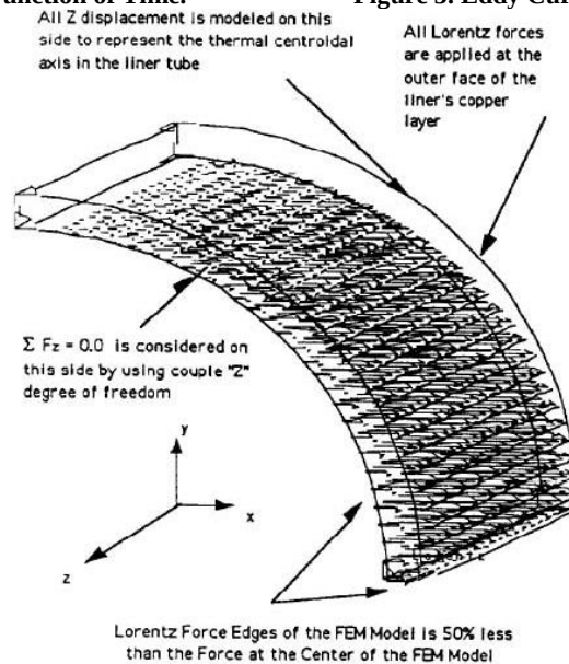
Figure 4. SSC Dipole Liner Tube FEM Model.
