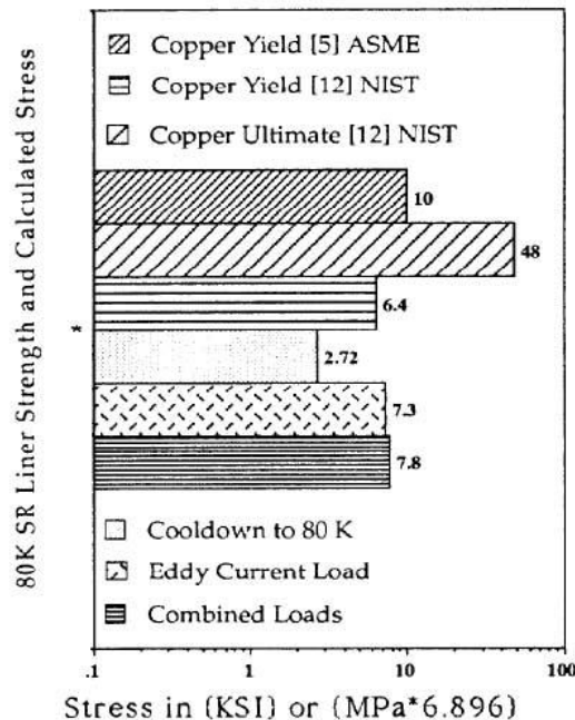
Figure 7. Result of Copper Layer Stress.
