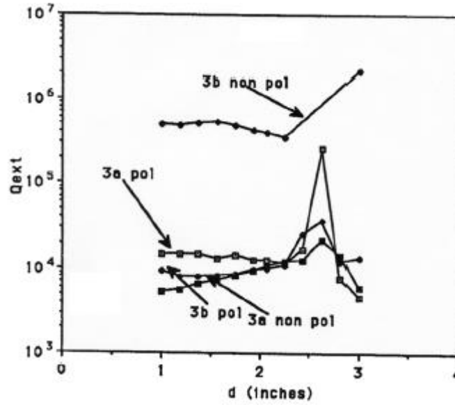
Fig. 2 Measured variations in Q_{ext} from changes in length of matching stub opposite single arm waveguide coupler.
