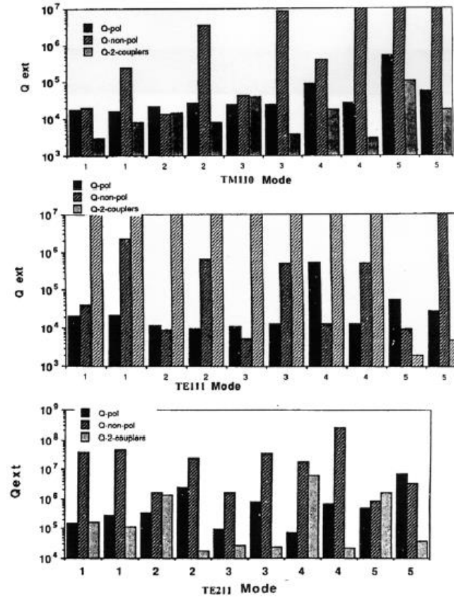
Fig. 3 Measured Q_{ext} for 3 deflecting mode pass-hands, TM_{110} , TE_{111} , and TE_{211} . There are 10 modes for each family. For each mode, Q_{ext} values for 3 different cases are given: polarized 5-cell cavity/one coupler, non-polarized 5-cell/one coupler, and the reference 5-cell LE-5 cavity with two arm couplers[3]. In the last case, only the Q_{ext} attributed to the HOM couplers is included.
