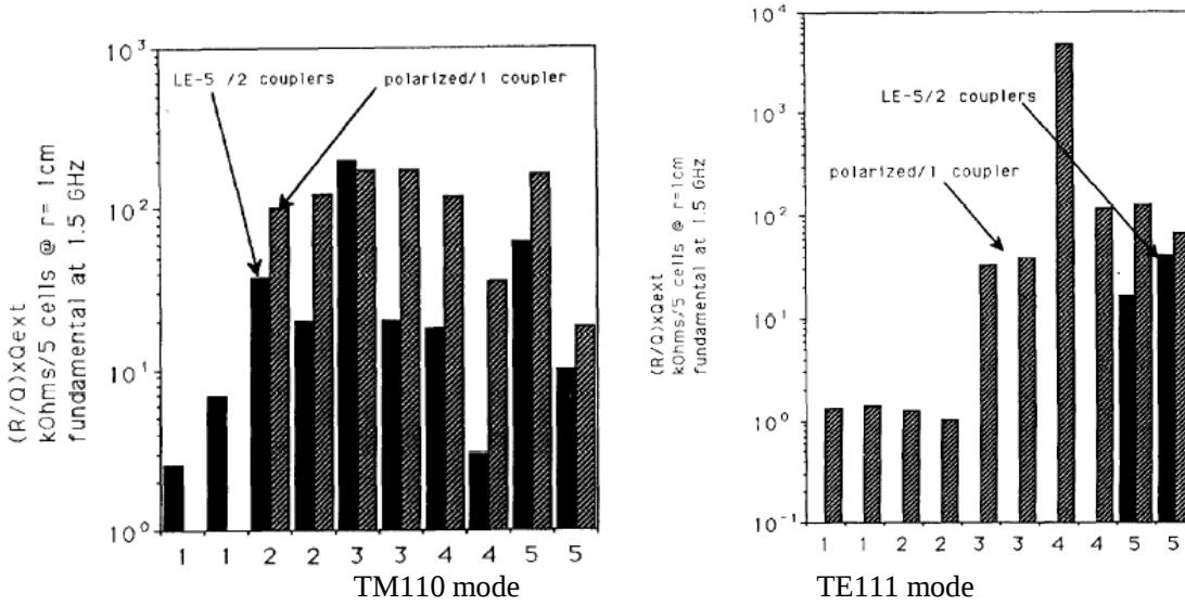
Fig. 4 Impedances, (R/Q) \times Q_{ext} , for the most dangerous dipole mode families: TM110 and TE111. Comparisons are made between the polarized /single coupler cavity and the reference LE-5 cavity (two couplers). For the TM110 mode family, the impedance values for the first two modes in the polarized cavity are too small to appear in the bar chart. For the TE111 family, the impedance of the first 8 modes for the reference cavity are left out as the two-arm HOM coupler does not provide any damping for these modes ( Q_{ext} = \infty ).
