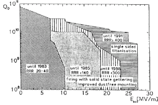
Fig.1: Performance limits of 3-GHz single cell cavities at Wuppertal ( T_{\text{Bath}}=1.5 K). Similar results have been obtained at 1.5 GHz [10]. ( \text{RRR} \approx 4 \cdot \lambda (4.2 K) [W/m \cdot K])
