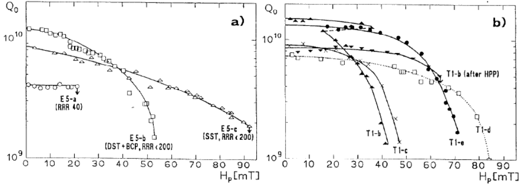
Fig.3: Q(H_p) performance of multicell 3 GHz cavities, a) 5-cell structure for SDALINAC b) 9-cell prototype for TESLA (Details on the preparation are given in the text.)
