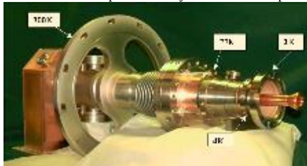
Figure 3: General assembly of TESLA coupler developed by AMAC
