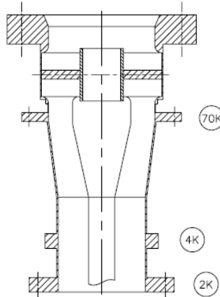
Figure 5: Cold window subassembly for AMAC TESLA coupler
