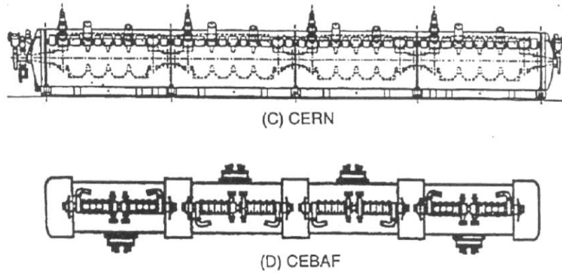
Figure 4. Cryomodules of the representative SRF structures in successful operation
