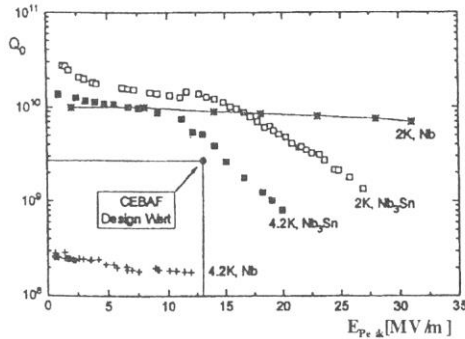
Figure 16. Initial results from a Nb 3 Sn cavity.
