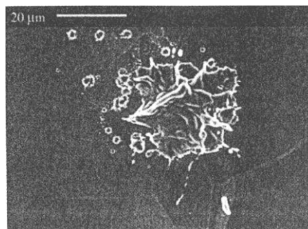
Figure 15. An emitter remained field of E_{pk}=17 MV/m.
