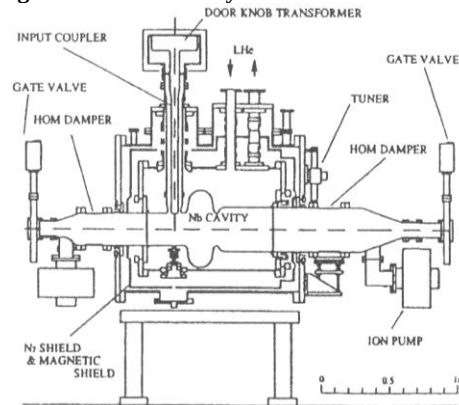
Figure 6. The layout of a cryomodule for the KEK-B SRF cavity.
