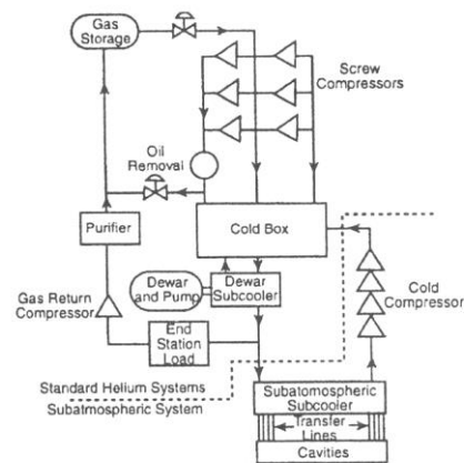
Fig. 13. A block diagram of the Refrigerator
