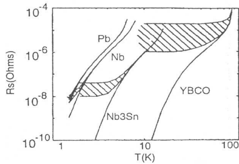
Figure 17. Surface resistances as functions of the temperatures for several LTc and HTc materials.
