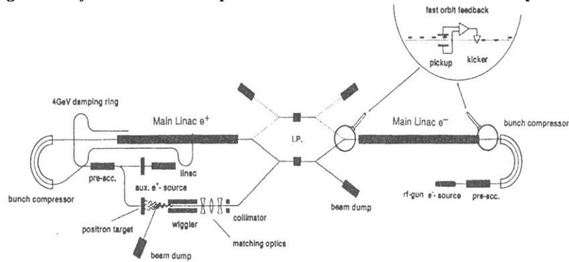
Figure 5. An overall layout of TESLA-500.
