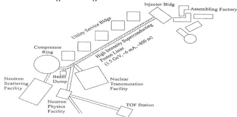
Figure 8. Plan of a facility layout for Proton Linac at JAERI (Japan)
