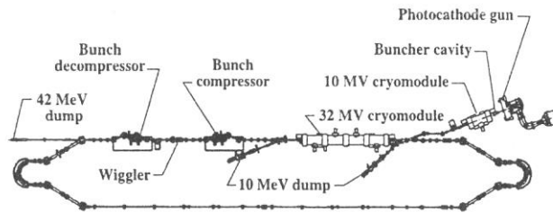
Figure 7. A schematic layout of the Jefferson Lab 1-kW IRFEL.
