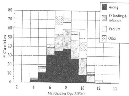
Figure 10. Performance of the CEBAF cavities in operation. TESLA in operation. HPR & HT
