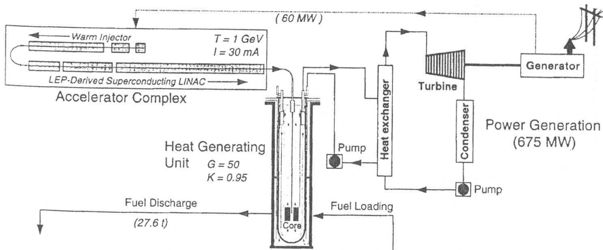
Figure 9. An energy amplifier with an SRF linac.
