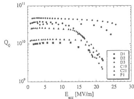
Figure 11. Performance of the cavities after HPR, HPP & HT
