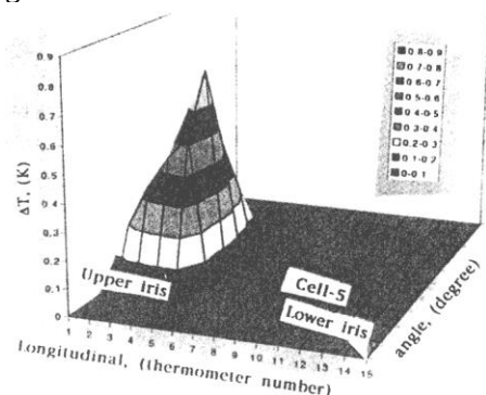
Figure 14. Identification of a TB location active at the at 12 MV/( E_{acc} ) on a TESLA cavity surface.
