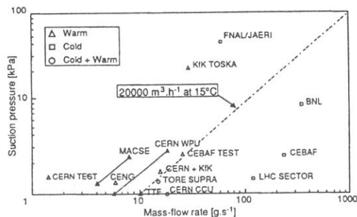
Fig. 12. Application range of the low-pressure He compressors.
