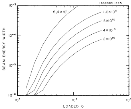
Fig. 4. The normalized beam energy width \sigma_{beam}^n is shown as a function of loaded Q for different values of the bunch charge. The mode bandwidth \Delta f/f = 2 \times 10^{-5}
