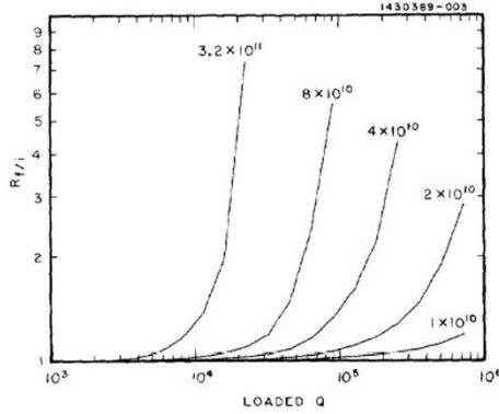
Fig. 1. The ratio R_{f/i} defined in (2) is shown as a function of the loaded Q of the mode. The mode impedance is (\frac{R}{Q}) = 1.3 \times 10^6 \Omega / \text{m}^3 .
