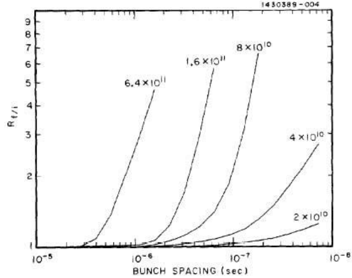
Fig. 3. The ratio R_t/i , is shown as a function of the bunch spacing for several values of the charge. The mode bandwidth is \Delta f/f = 2 \times 10^{-5} . There are 10 distinct modes in each cavity.
