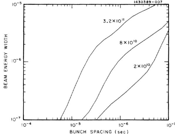
Fig. 6. The normalized beam energy width \sigma_{beam}^n is shown as a function of bunch spacing for various values of the bunch charge. \Delta f / f = 2 \times 10^{-5} . There are ten modes in each cavity.
