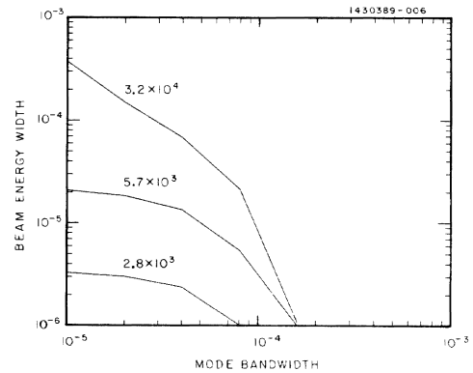
Fig. 5. \sigma_{beam}^n is shown as a function of the bandwidth for different values of the loaded Q for 4 \times 10^{10} particles per bunch.
