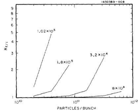
Fig. 2. The ratio R_{f/i} is shown as a function of the bunch charge. The beam emittance growth is indicated for several values of
