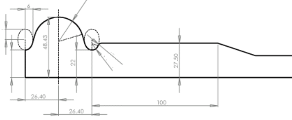
Fig 3: Cavity configuration after several series of Optimization
