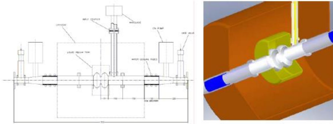
Fig 1: A schematic of the 2.85 GHz SRF cavity with a high RF power input coupler and HOM absorber
