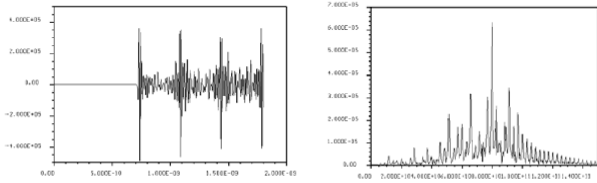
Fig 5. Examples: RF electric field at point 1 & frequency spectrum induced by 6 bunches
