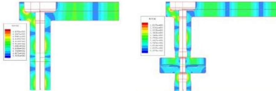
Fig. 6. Straight Coaxial RF Coupler Section and Tapered Coaxial Coupler Section.
