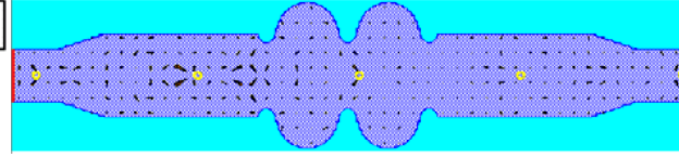
Fig 4: 6 Bunches are passing the cavity (the 1 st one has passed through).
