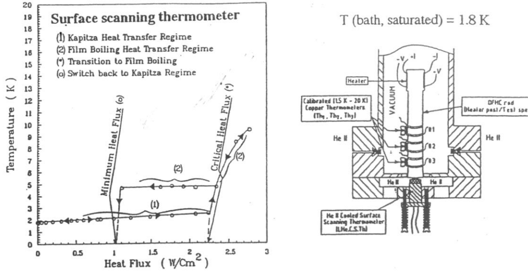
Figure 2. Scheme of a device for study of surface heat wander in LHe II; (B) Heat transfer between a heart surface and He II with large heat fluxes. The transition between the Kapitza regime and film boil is identified.
