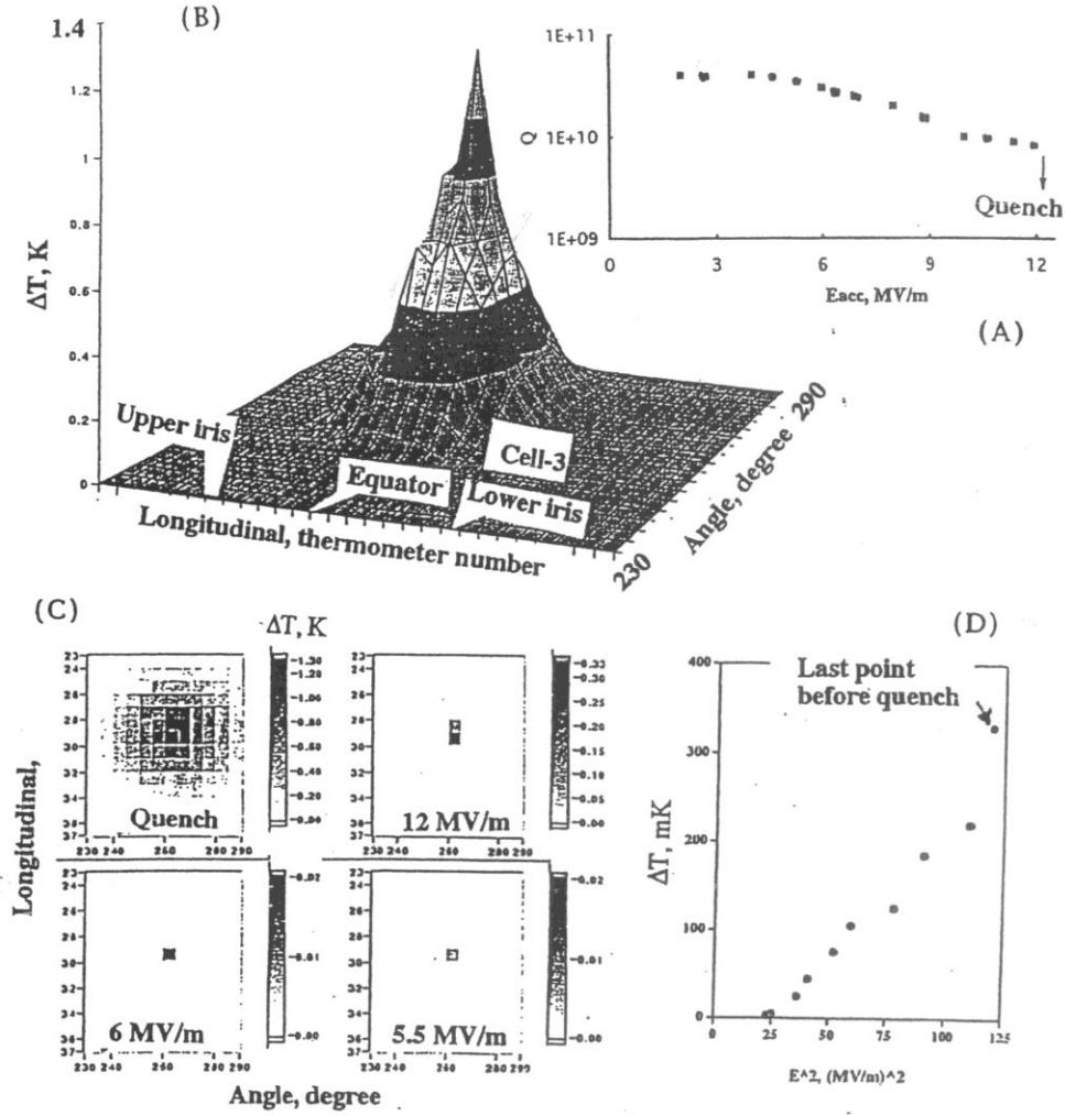
Figure 1.(A) Overall RF performance of cavity D-4; (B) The beaten area of cavity D-4 during quench at 12 MV/m in He II; (C) T maps during and before quench; (D) \Delta T at the quench origin as a function of (E_{acc})^2 before quench.
